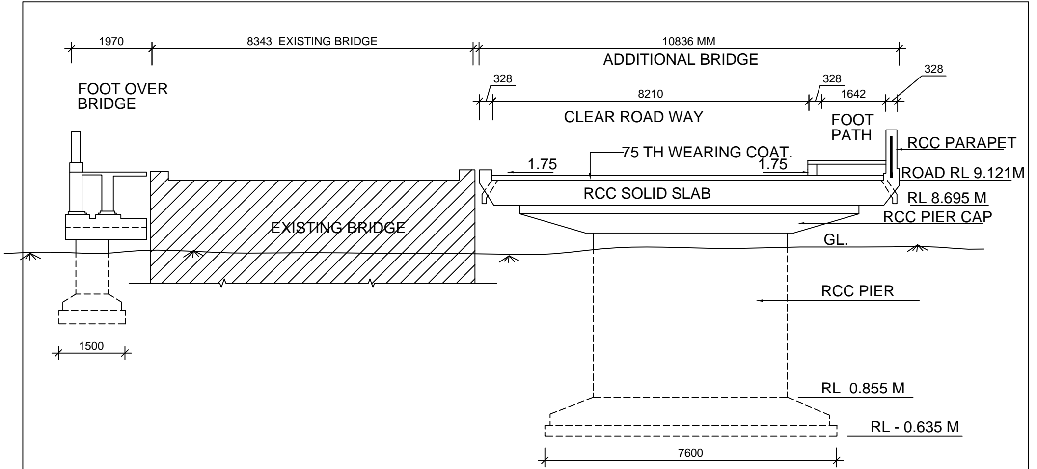
CROSS SECTION (SKEW)
