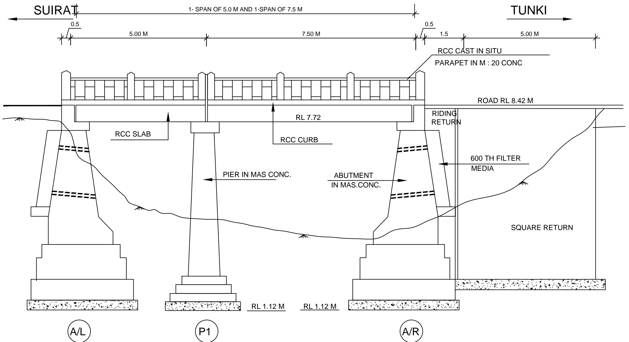
SECTIONAL ELEVATION
