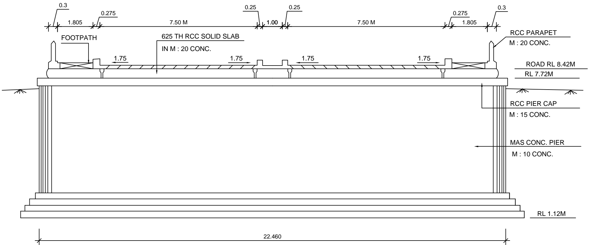
CROSS SECTION
