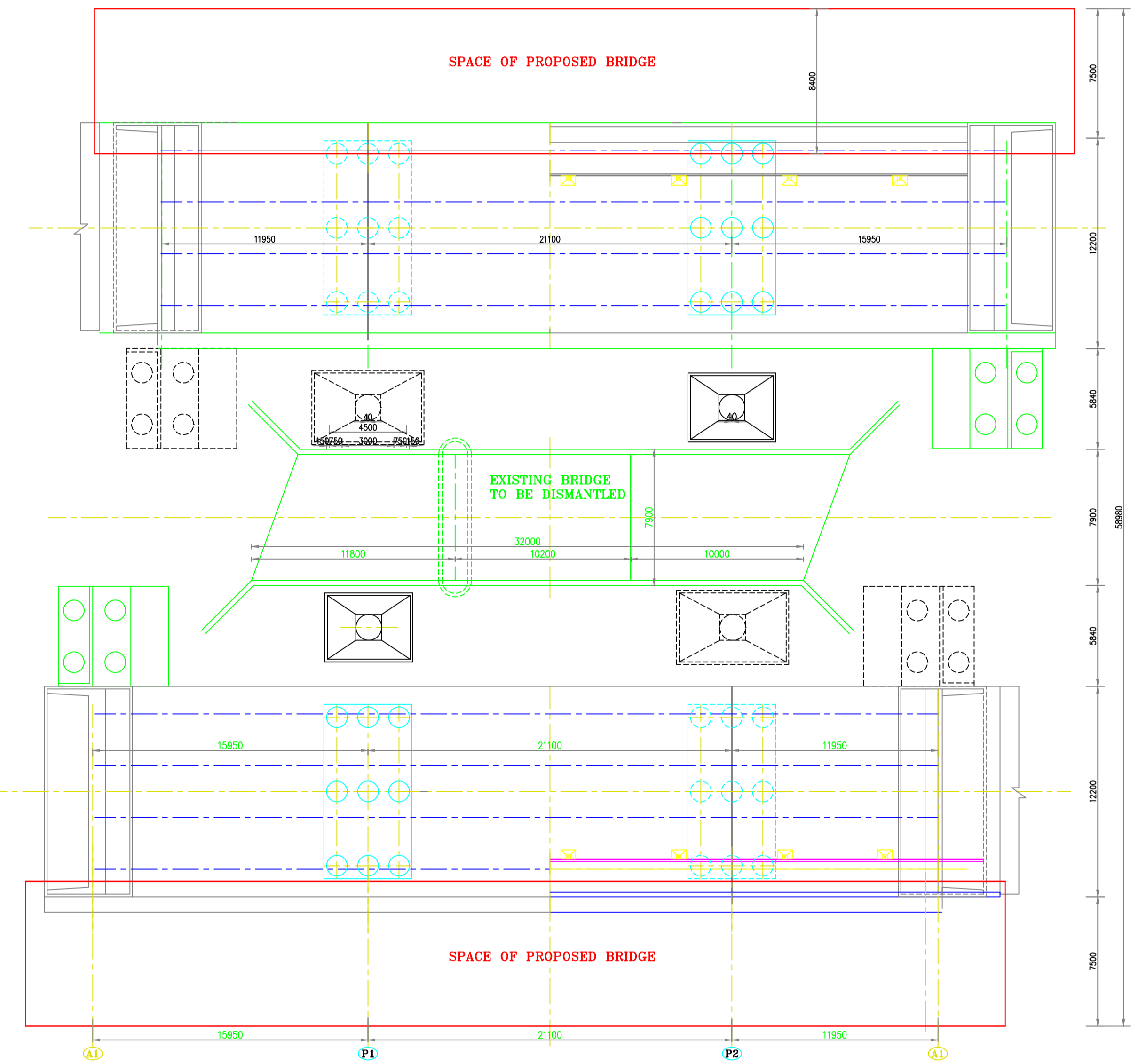
PLAN SHOWING DETAILS OF EXISTING BRIDGE SCALE: 1:200
