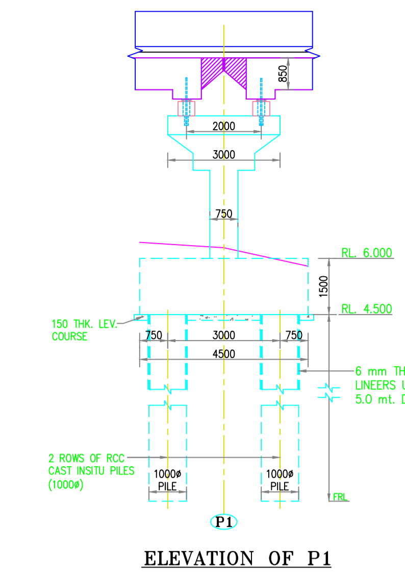
ELEVATION OF P1
