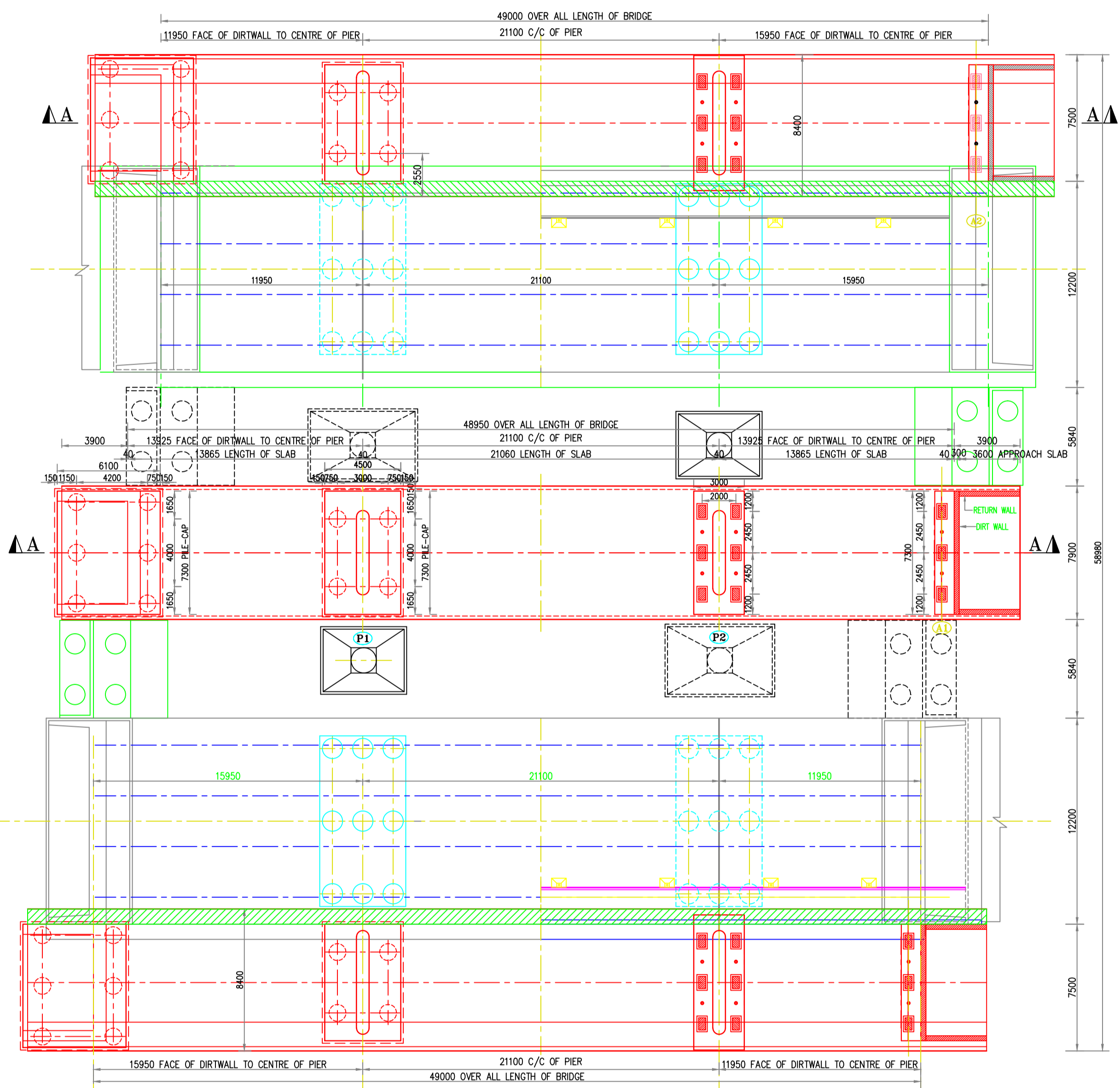
PLAN SHOWING DETAILS OF PROPOSED BRIDGE SCALE: 1:200
