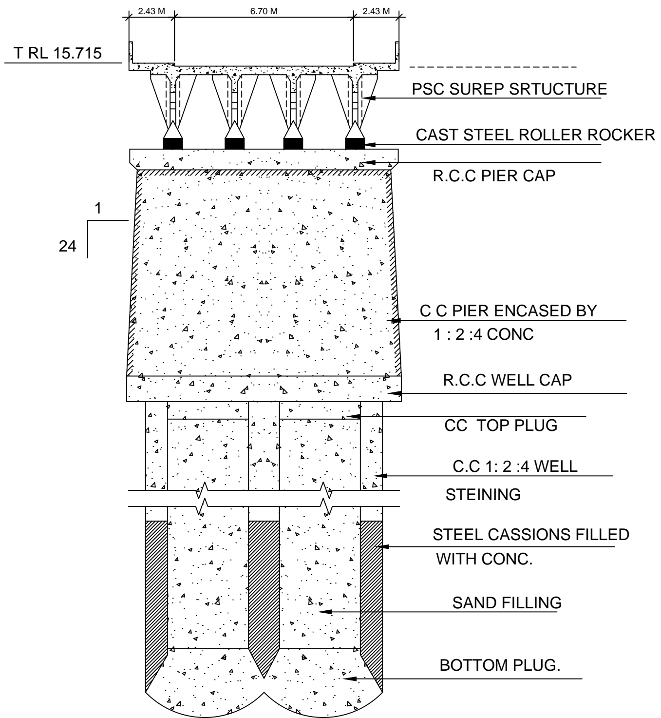
CROSS SECTION
