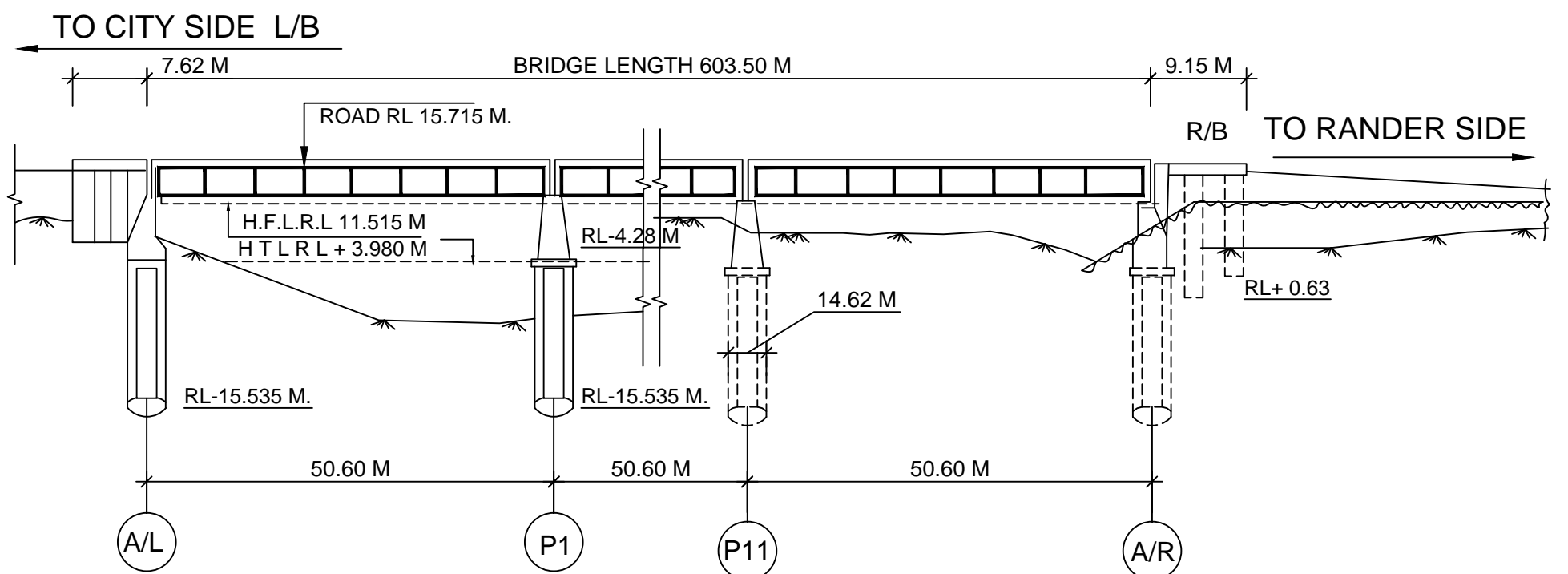
SECTIONAL ELEVATION
